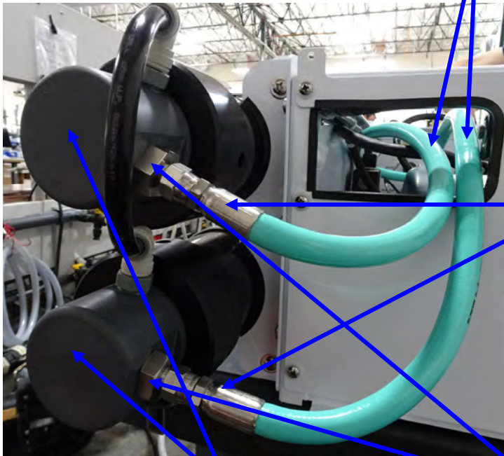
FT-PV-EC4IN SPECTRA 4" PRESSURE VESSEL END CAP
