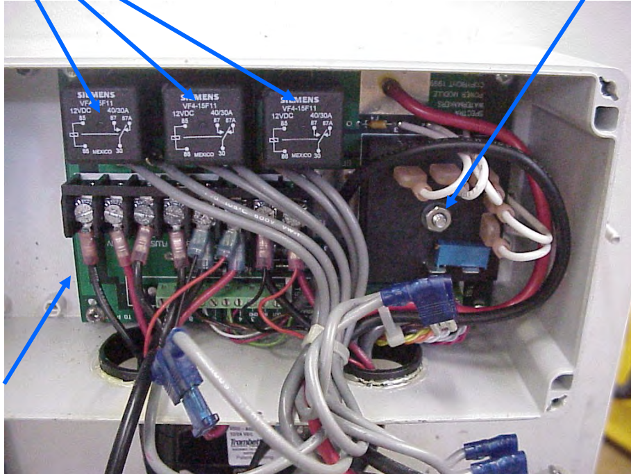
EL-ELM-CPCB Main Circuit Board
