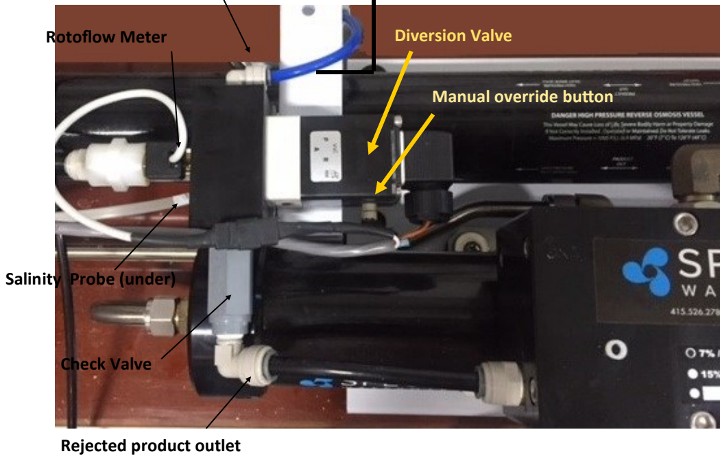
Product Diversion Valve Manifold
