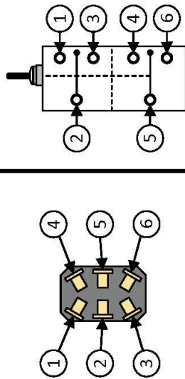
Detail View: DPDT Switch Operational Schematic
